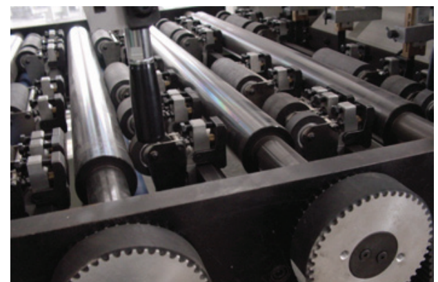
Fixed foil puller system, foil change outside of the machine
